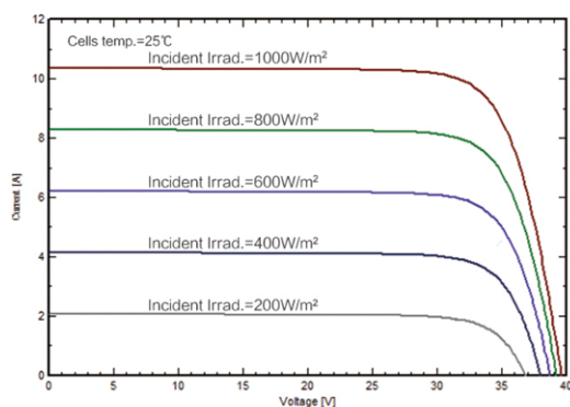
I-V Curve at different irradiation
